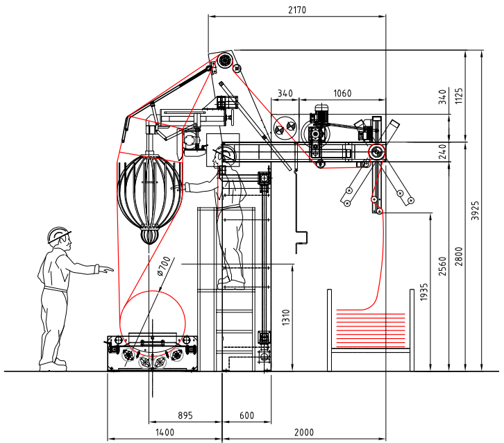
The Bianco® Simple Slitter on fold
