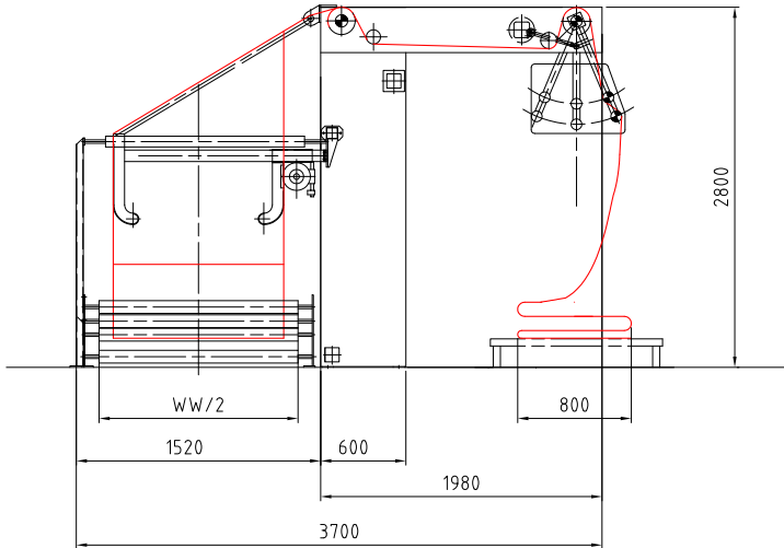
The Bianco® Simple Slitter on fold
