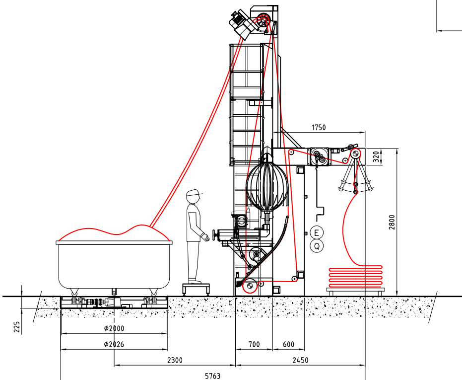
Bianco® Reverse Slitter
